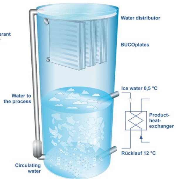
BUCOdelot ice-store Falling-Film - Ice-maker
